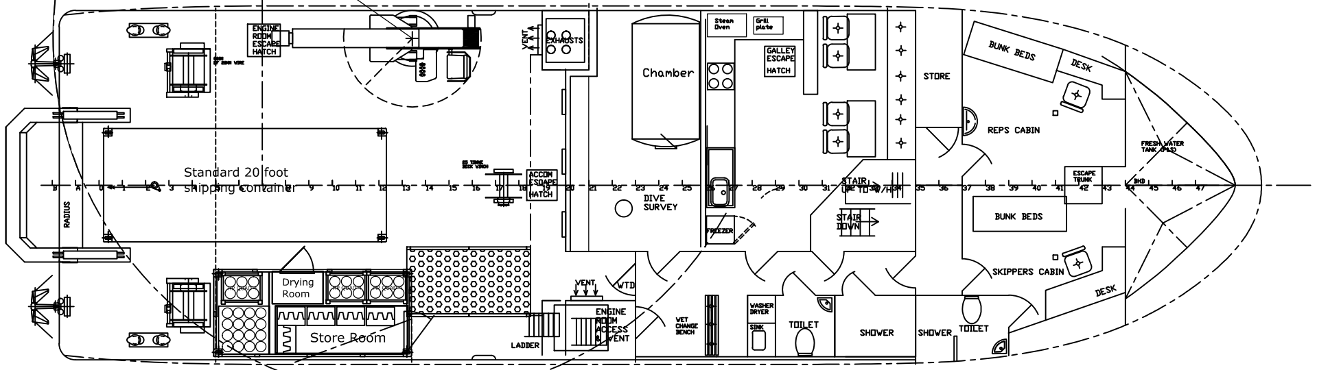
PLAN ON MAIN DECK
